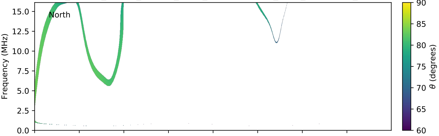
expres_cassini_jupiter_europa_isaac_lossc-wid1deg_3kev_20010127_v01.cdf
