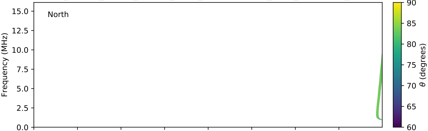
expres_cassini_jupiter_europa_isaac_lossc-wid1deg_3kev_20010126_v01.cdf
