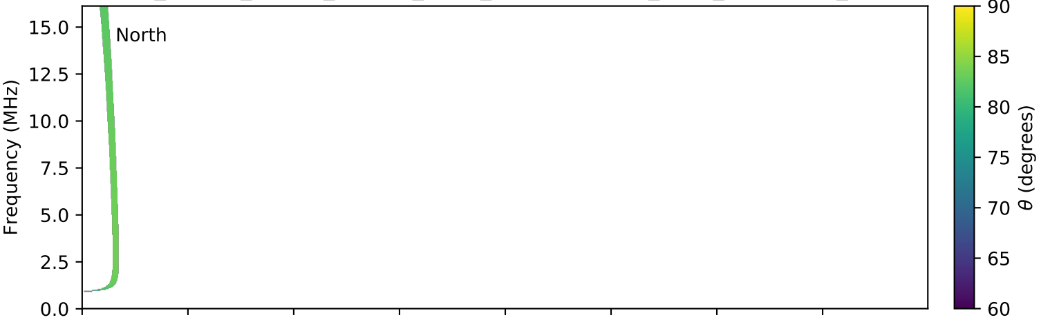
expres_cassini_jupiter_europa_isaac_lossc-wid1deg_3kev_20010125_v01.cdf
