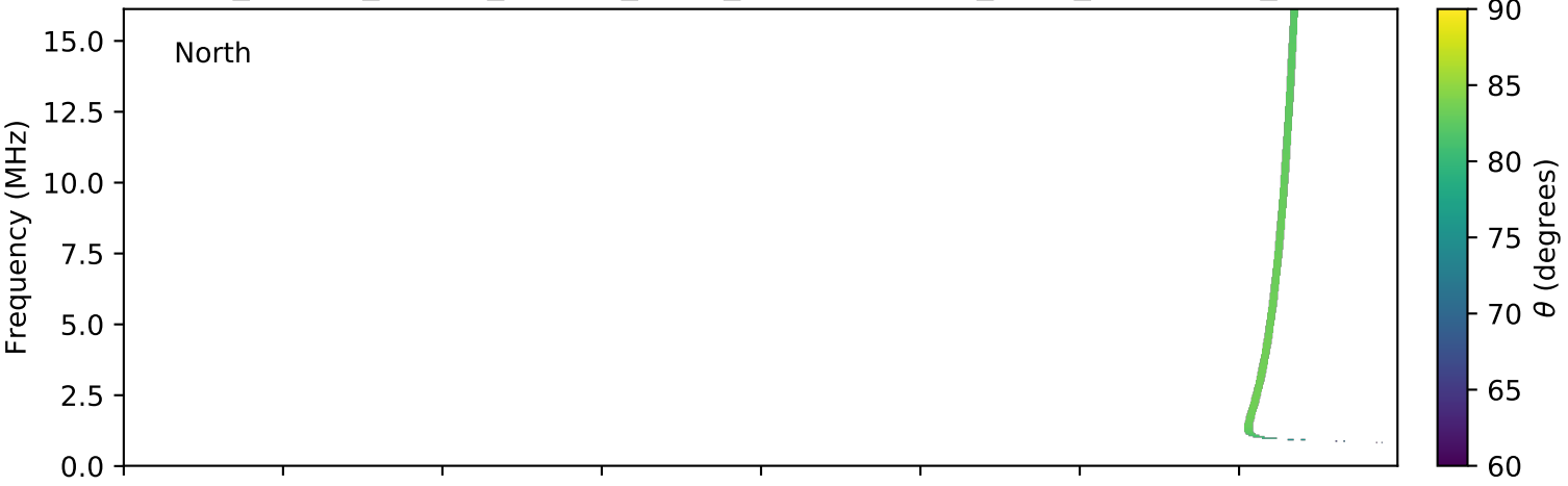
expres_cassini_jupiter_europa_isaac_lossc-wid1deg_3kev_20010119_v01.cdf
