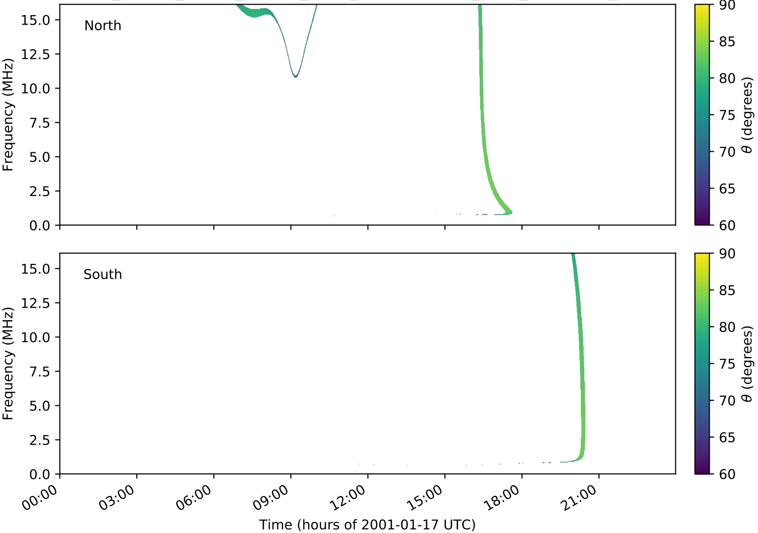
expres_cassini_jupiter_europa_isaac_lossc-wid1deg_3kev_20010117_v01.cdf
