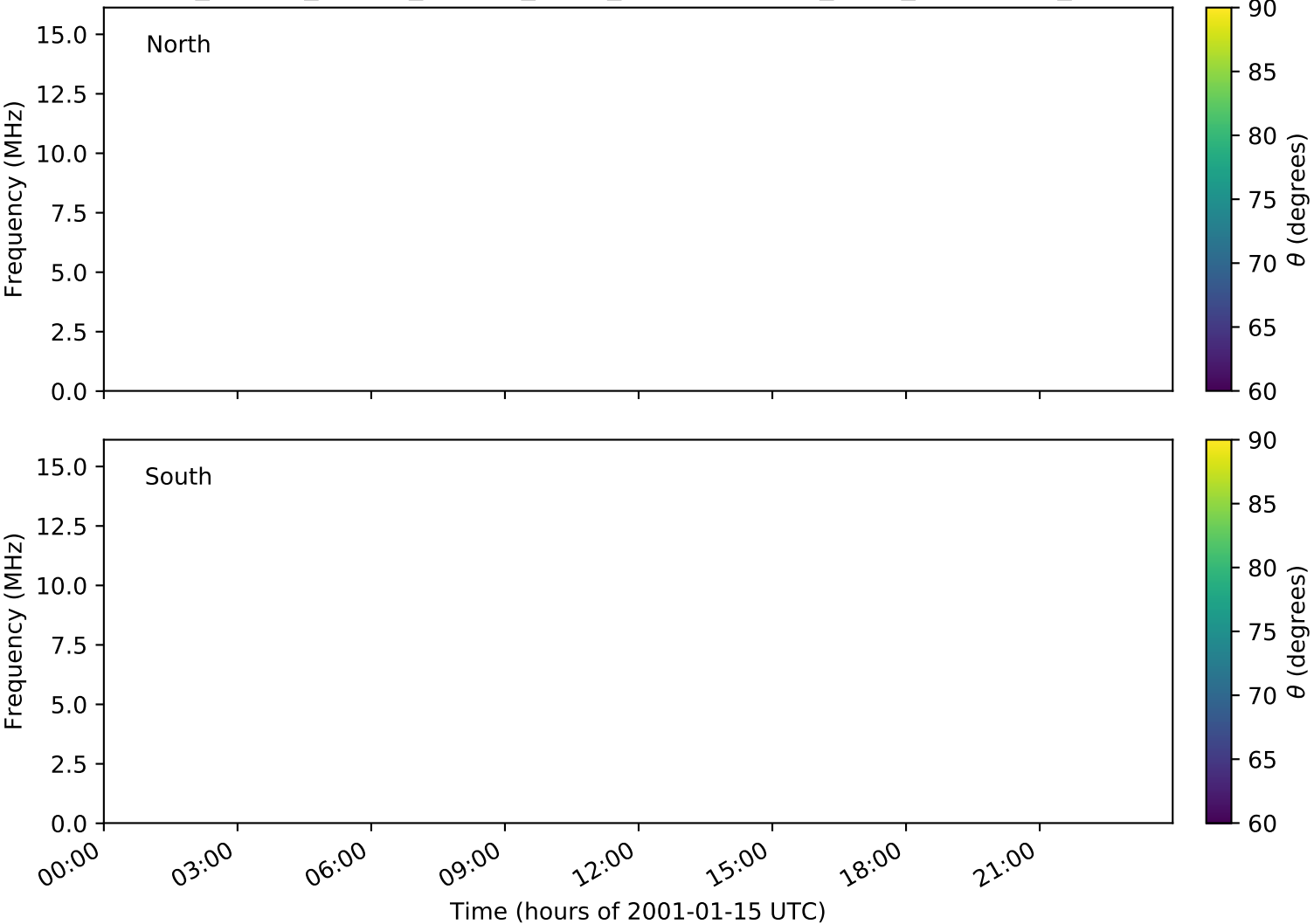
expres_cassini_jupiter_europa_isaac_lossc-wid1deg_3kev_20010115_v01.cdf
