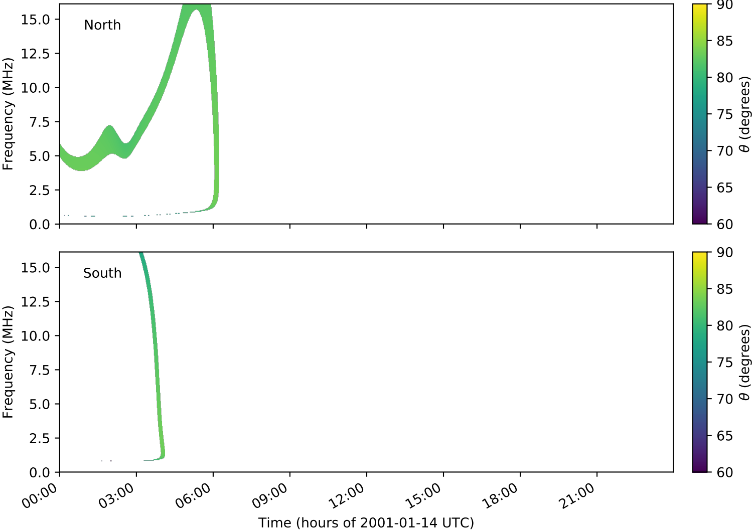
expres_cassini_jupiter_europa_isaac_lossc-wid1deg_3kev_20010114_v01.cdf
