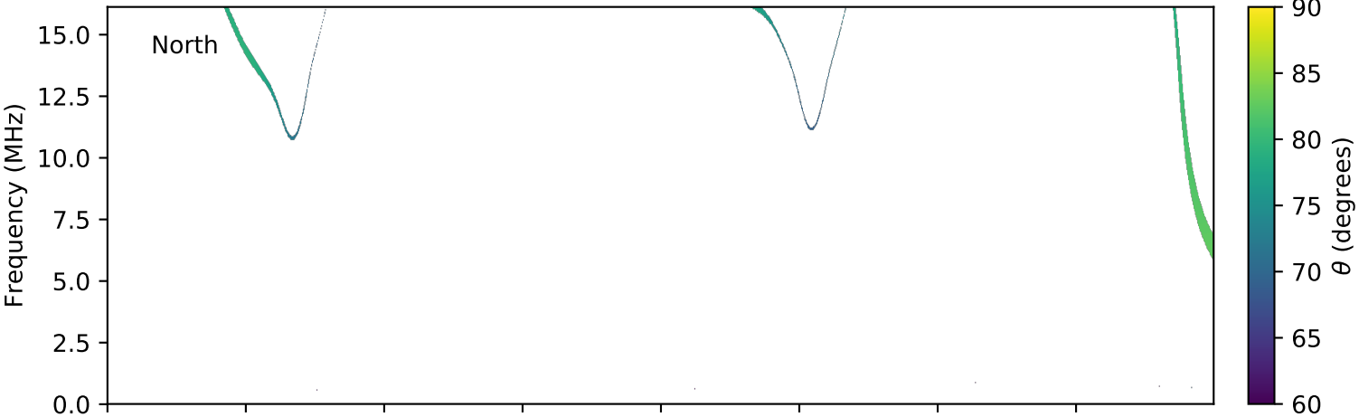
expres_cassini_jupiter_europa_isaac_lossc-wid1deg_3kev_20010113_v01.cdf
