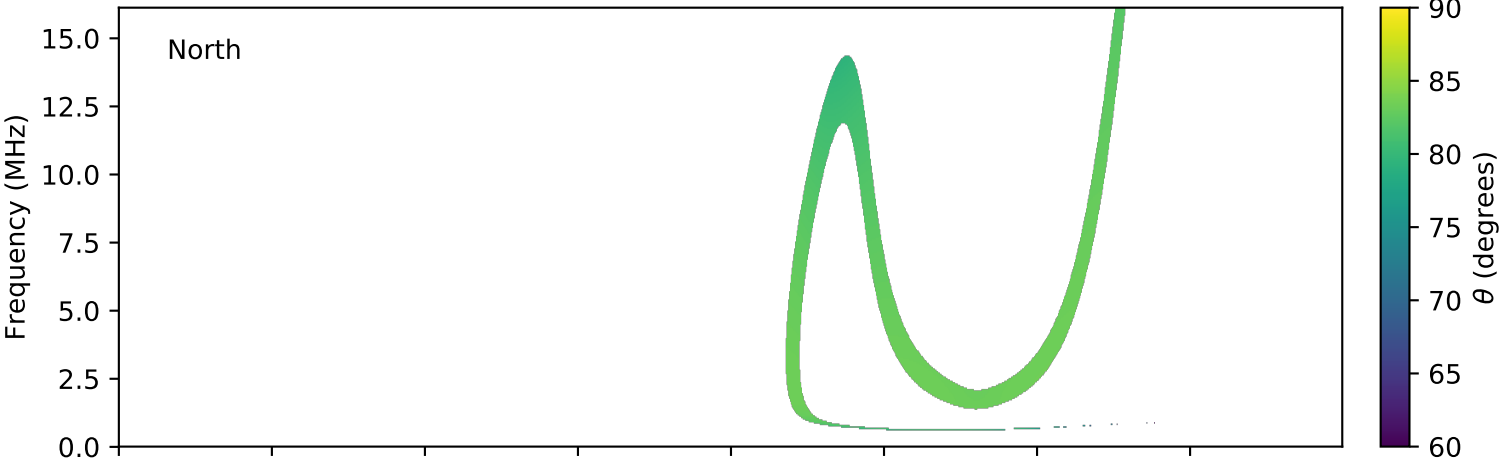
expres_cassini_jupiter_europa_isaac_lossc-wid1deg_3kev_20010112_v01.cdf
