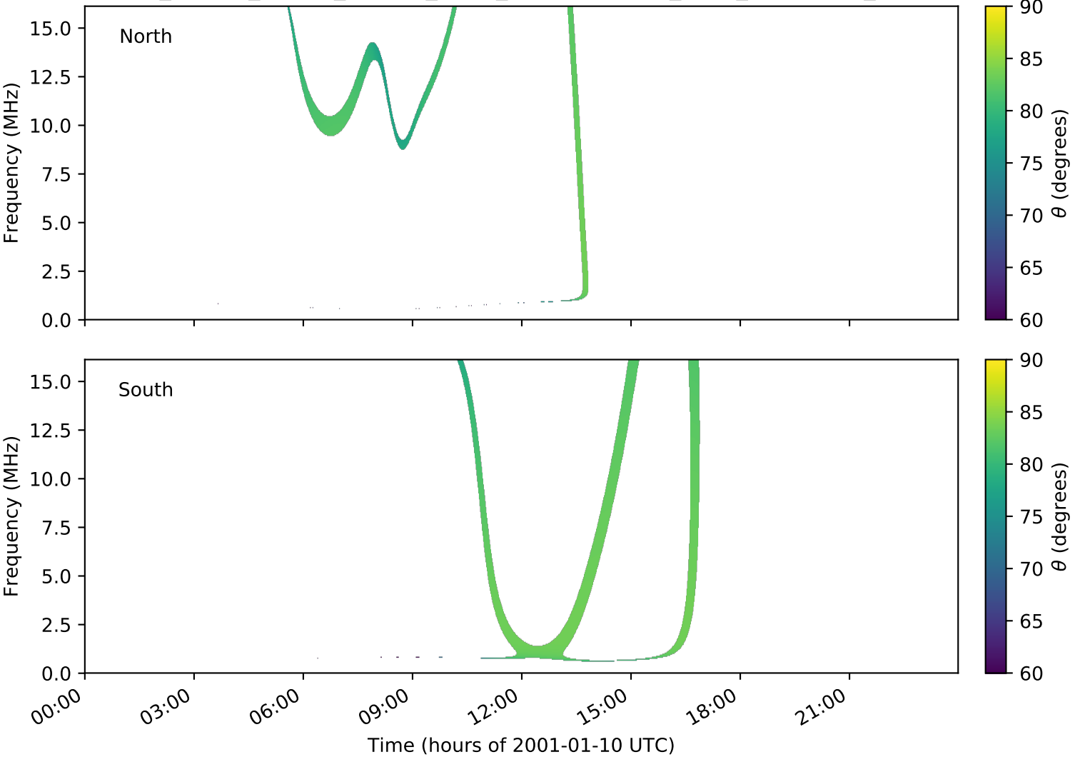
expres_cassini_jupiter_europa_isaac_lossc-wid1deg_3kev_20010110_v01.cdf
