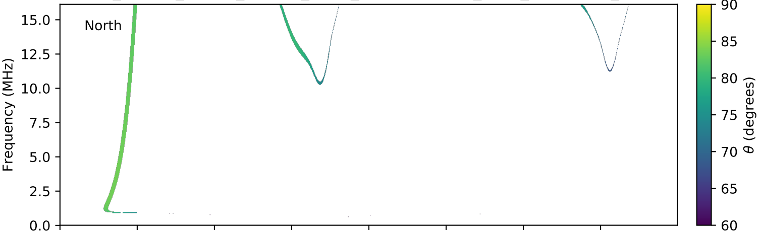
expres_cassini_jupiter_europa_isaac_lossc-wid1deg_3kev_20010109_v01.cdf
