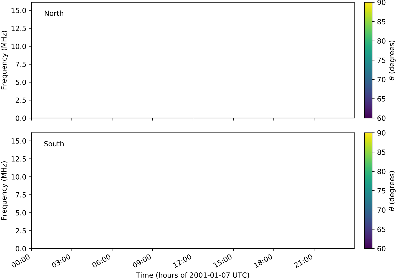
expres_cassini_jupiter_europa_isaac_lossc-wid1deg_3kev_20010107_v01.cdf
