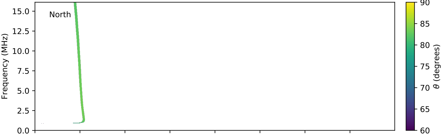
expres_cassini_jupiter_europa_isaac_lossc-wid1deg_3kev_20010103_v01.cdf
