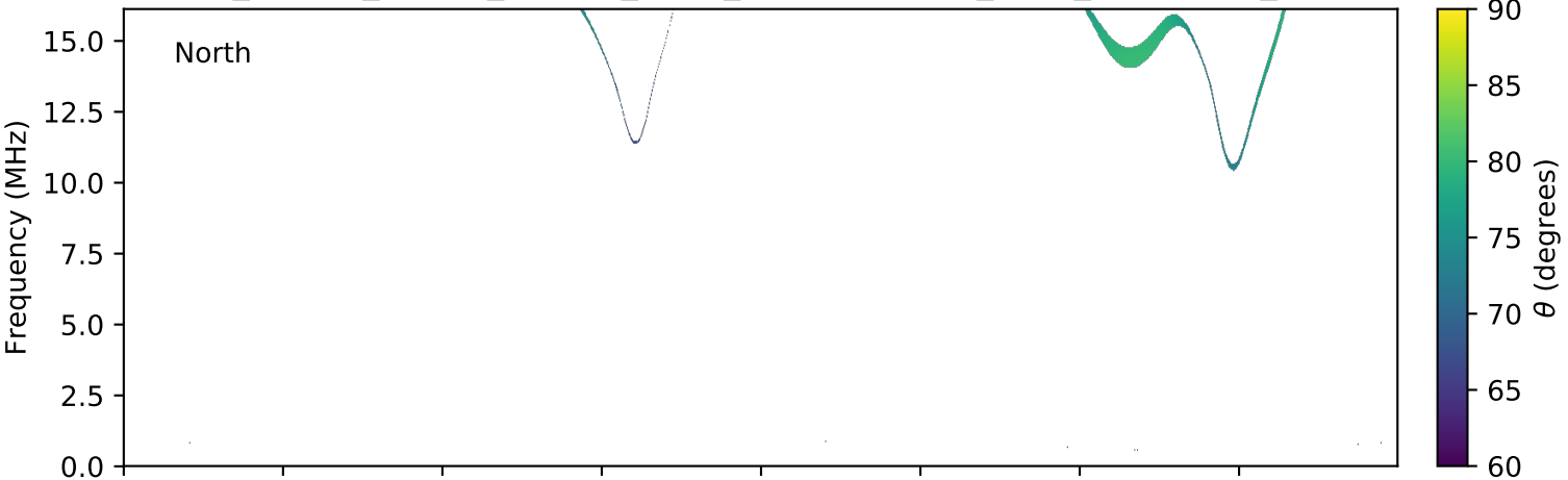
expres_cassini_jupiter_europa_isaac_lossc-wid1deg_3kev_20010102_v01.cdf
