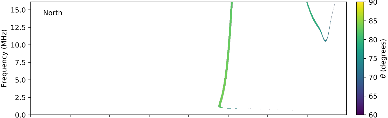
expres_cassini_jupiter_europa_isaac_lossc-wid1deg_3kev_20010101_v01.cdf
