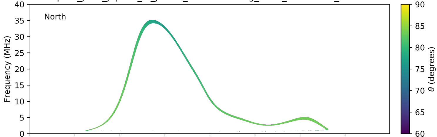
expres_juno_jupiter_io_jrm09_lossc-wid1deg_3kev_20211231_v11.cdf
