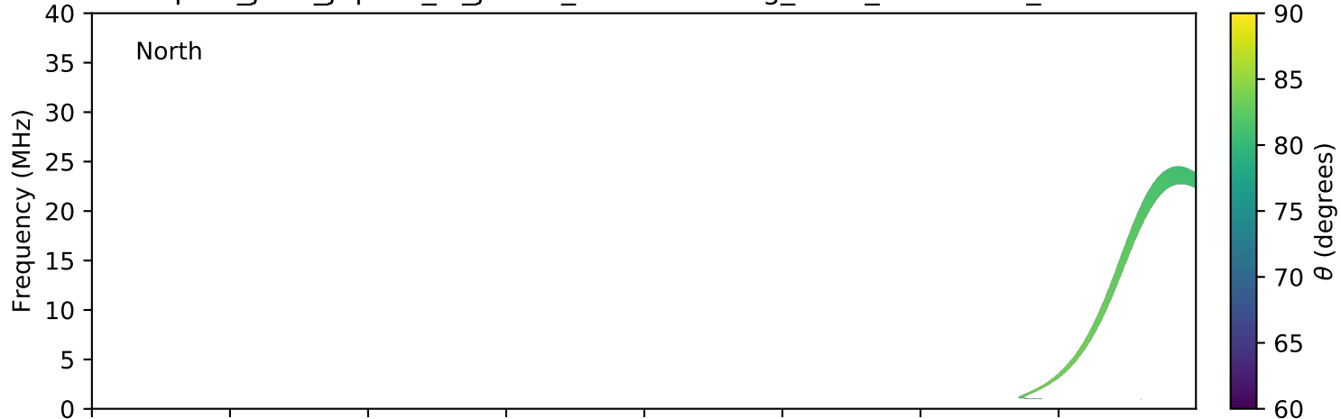
expres_juno_jupiter_io_jrm09_lossc-wid1deg_3kev_20211225_v11.cdf
