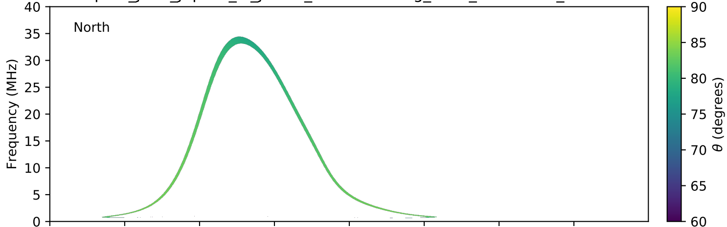
expres_juno_jupiter_io_jrm09_lossc-wid1deg_3kev_20211224_v11.cdf
