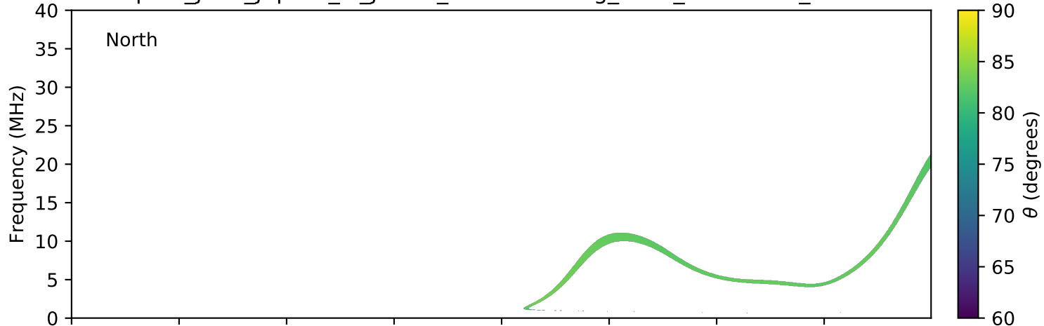
expres_juno_jupiter_io_jrm09_lossc-wid1deg_3kev_20211220_v11.cdf
