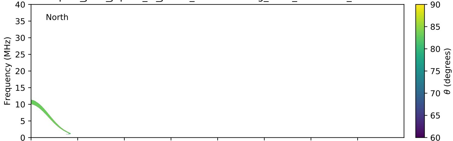
expres_juno_jupiter_io_jrm09_lossc-wid1deg_3kev_20211214_v11.cdf
