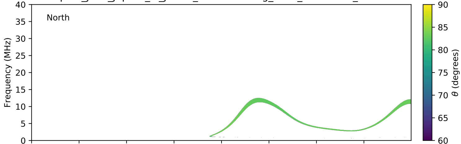
expres_juno_jupiter_io_jrm09_lossc-wid1deg_3kev_20211213_v11.cdf
