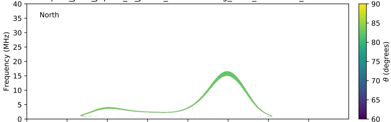
expres_juno_jupiter_io_jrm09_lossc-wid1deg_3kev_20211208_v11.cdf
