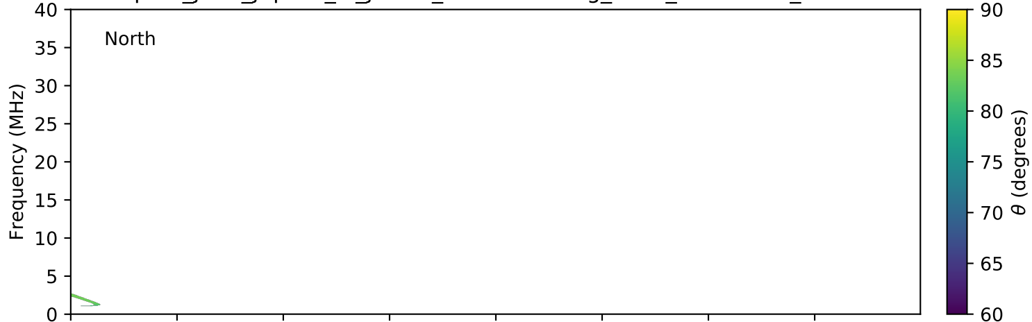
expres_juno_jupiter_io_jrm09_lossc-wid1deg_3kev_20211207_v11.cdf
