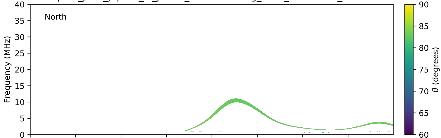
expres_juno_jupiter_io_jrm09_lossc-wid1deg_3kev_20211206_v11.cdf
