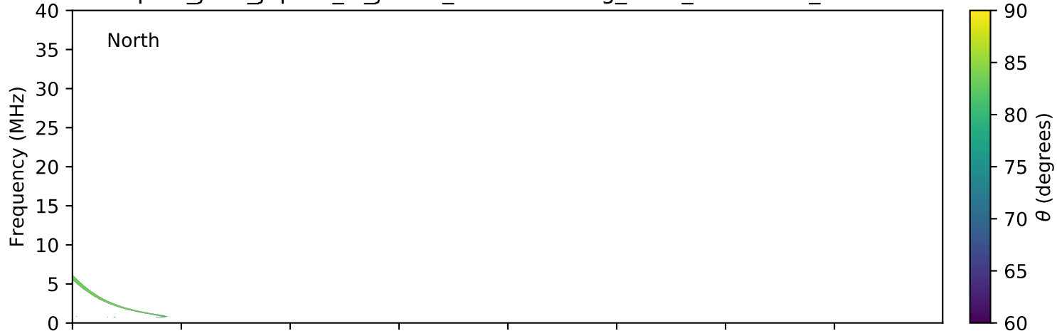
expres_juno_jupiter_io_jrm09_lossc-wid1deg_3kev_20211205_v11.cdf
