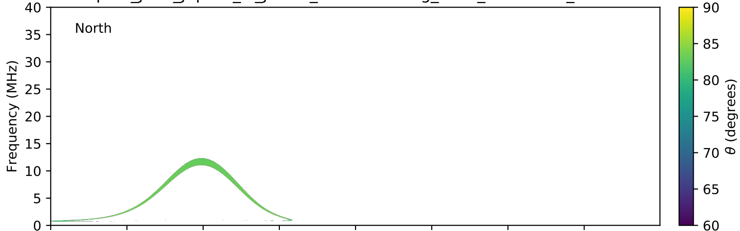
expres_juno_jupiter_io_jrm09_lossc-wid1deg_3kev_20211203_v11.cdf
