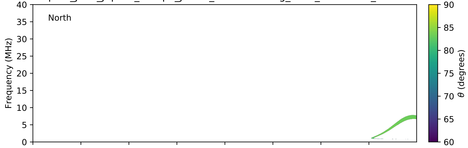
expres_juno_jupiter_europa_jrm09_lossc-wid1deg_3kev_20211225_v11.cdf
