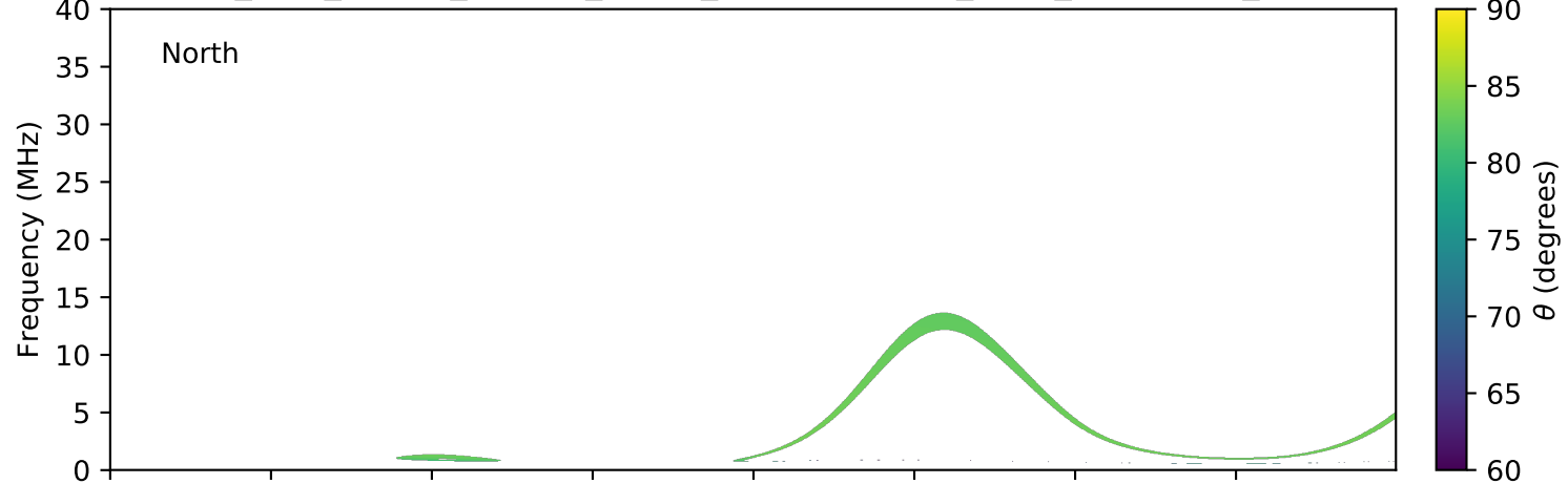
expres_juno_jupiter_europa_jrm09_lossc-wid1deg_3kev_20211215_v11.cdf
