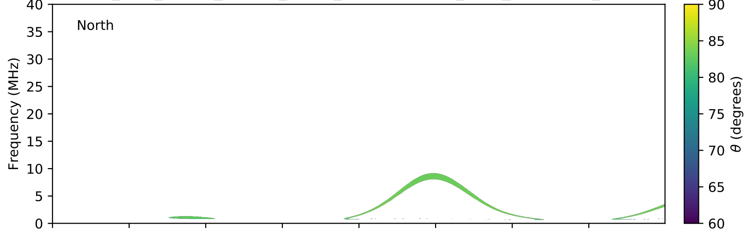
expres_juno_jupiter_europa_jrm09_lossc-wid1deg_3kev_20211208_v11.cdf
