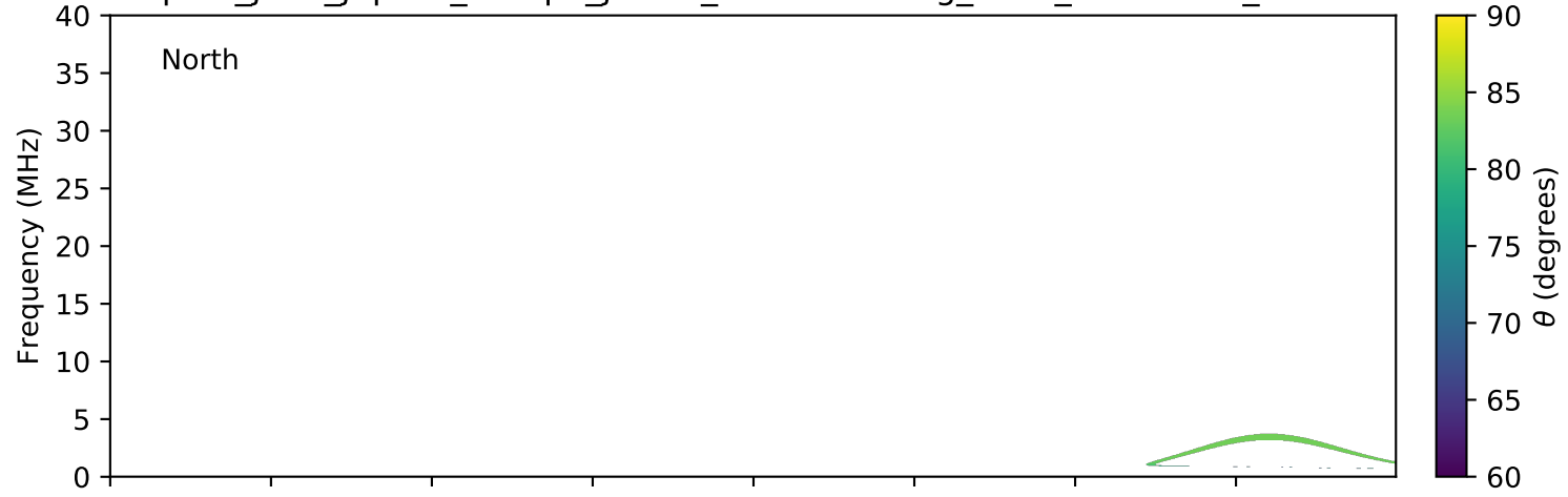
expres_juno_jupiter_europa_jrm09_lossc-wid1deg_3kev_20211204_v11.cdf
