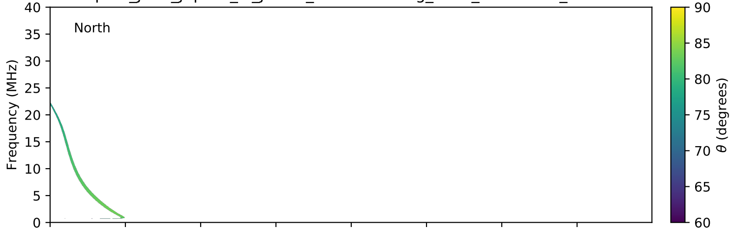
expres_juno_jupiter_io_jrm09_lossc-wid1deg_3kev_20211128_v11.cdf
