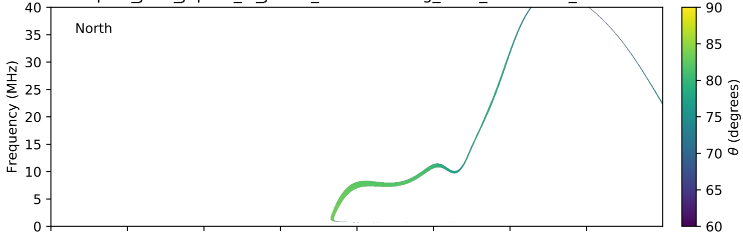
expres_juno_jupiter_io_jrm09_lossc-wid1deg_3kev_20211127_v11.cdf
