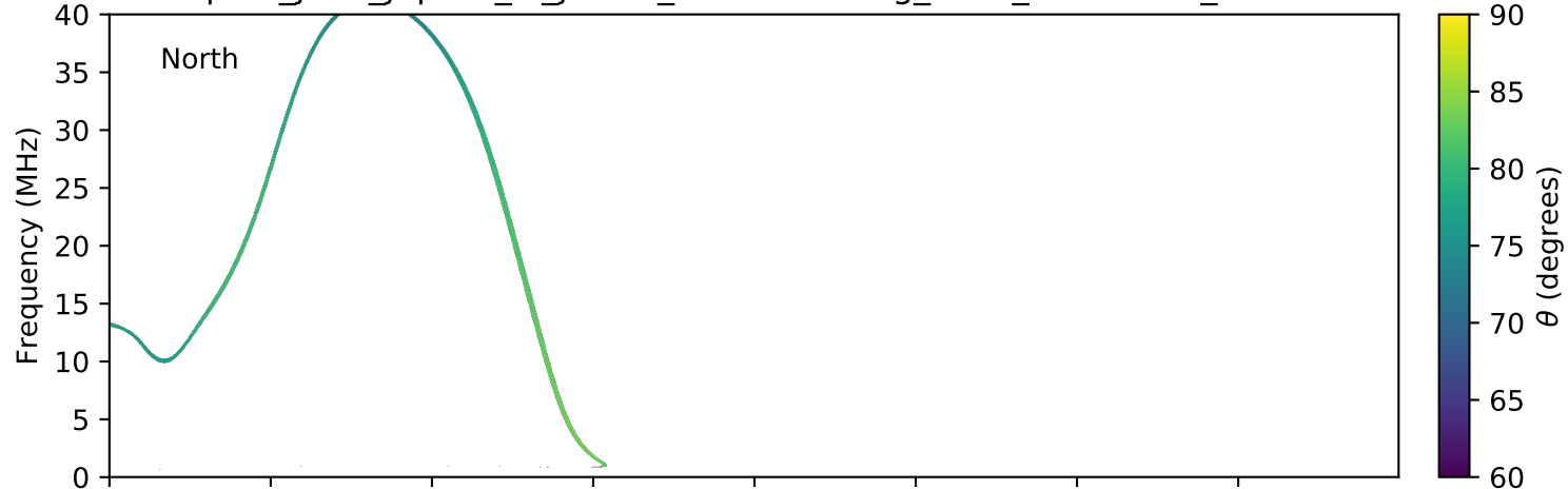
expres_juno_jupiter_io_jrm09_lossc-wid1deg_3kev_20211126_v11.cdf
