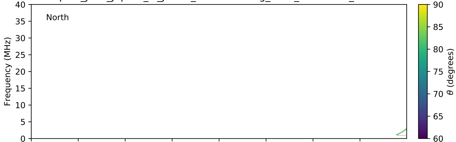
expres_juno_jupiter_io_jrm09_lossc-wid1deg_3kev_20211123_v11.cdf
