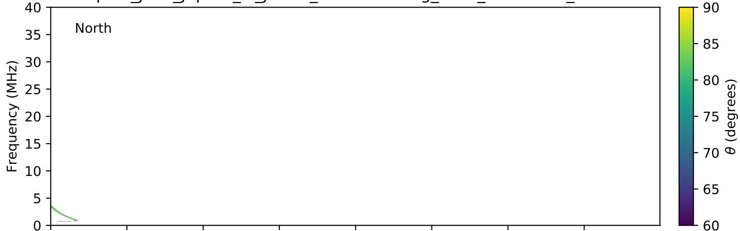
expres_juno_jupiter_io_jrm09_lossc-wid1deg_3kev_20211121_v11.cdf
