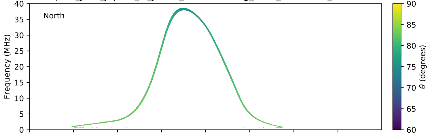
expres_juno_jupiter_io_jrm09_lossc-wid1deg_3kev_20211115_v11.cdf
