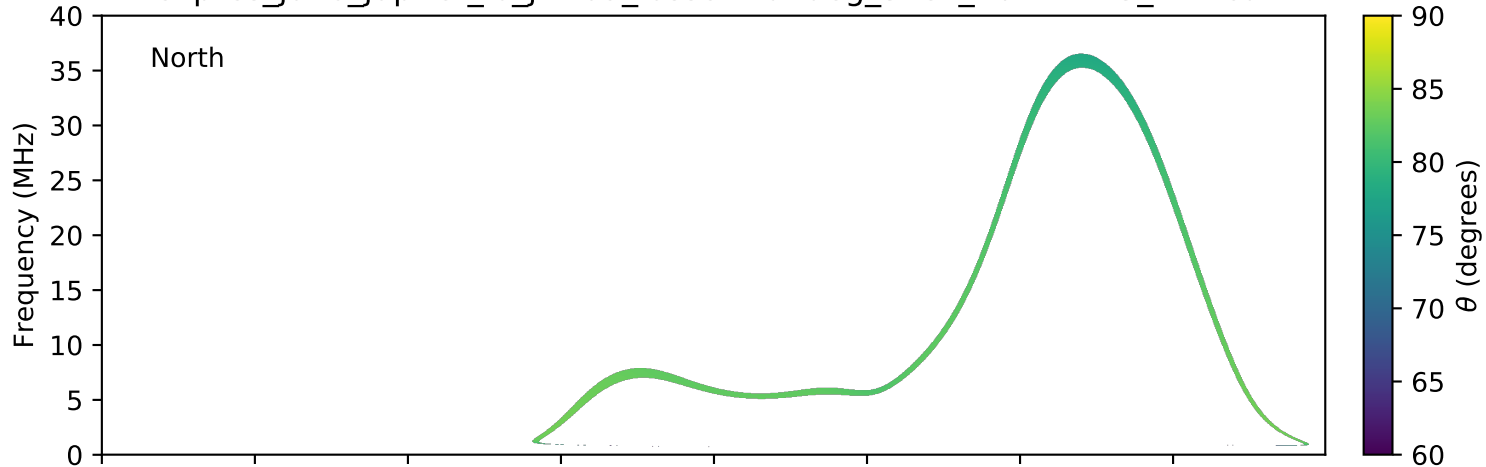
expres_juno_jupiter_io_jrm09_lossc-wid1deg_3kev_20211113_v11.cdf
