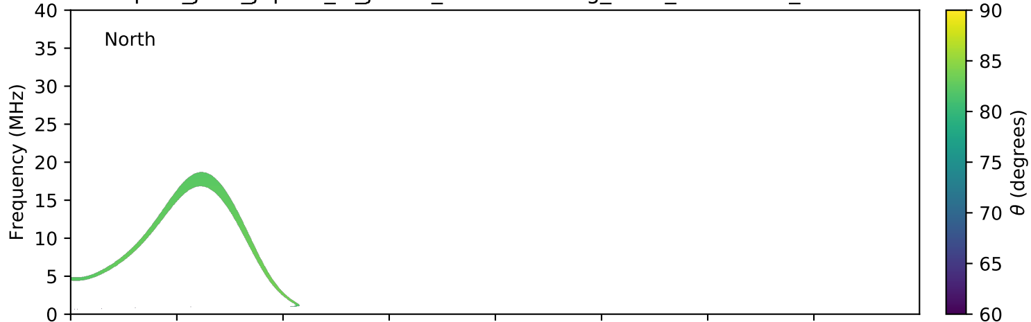
expres_juno_jupiter_io_jrm09_lossc-wid1deg_3kev_20211112_v11.cdf
