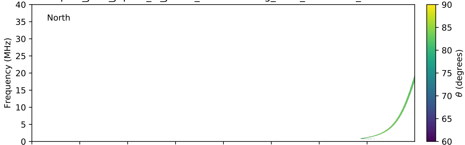
expres_juno_jupiter_io_jrm09_lossc-wid1deg_3kev_20211109_v11.cdf
