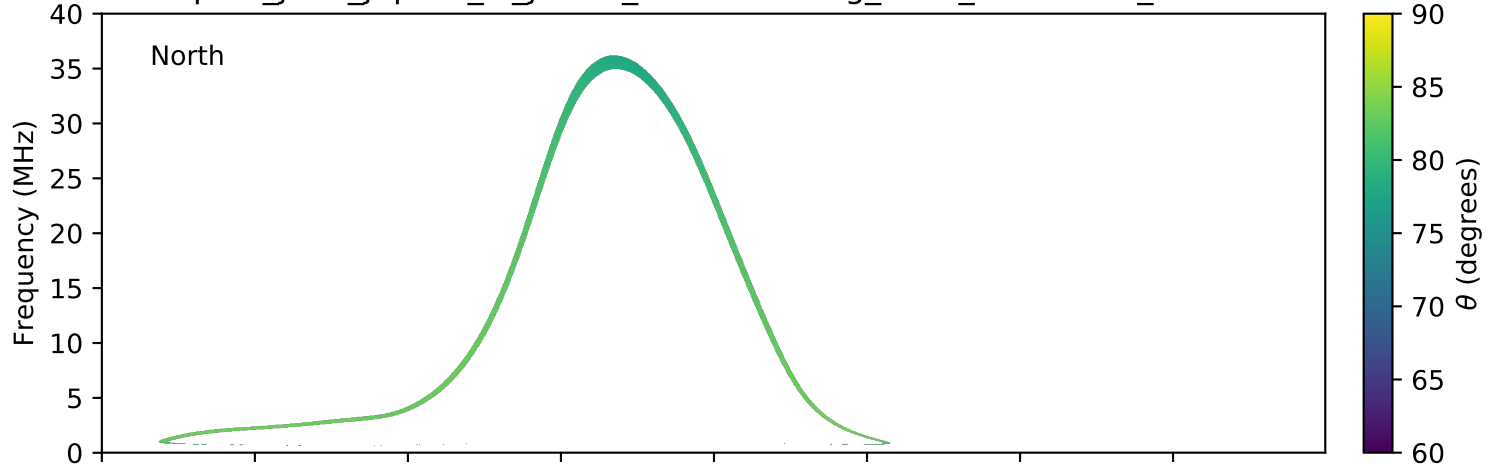
expres_juno_jupiter_io_jrm09_lossc-wid1deg_3kev_20211108_v11.cdf
