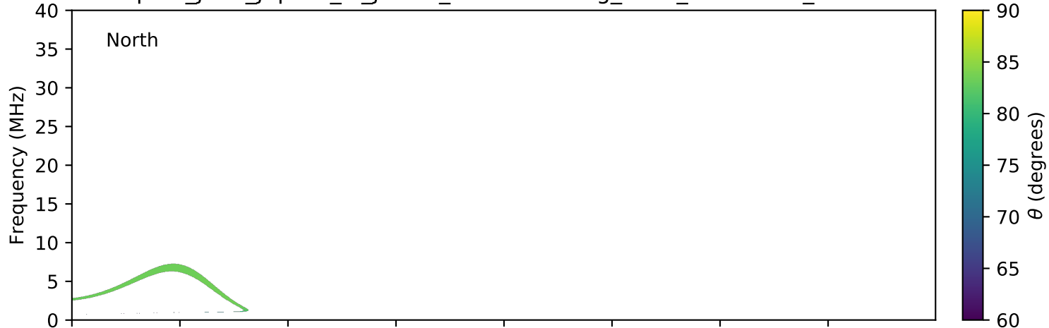
expres_juno_jupiter_io_jrm09_lossc-wid1deg_3kev_20211105_v11.cdf
