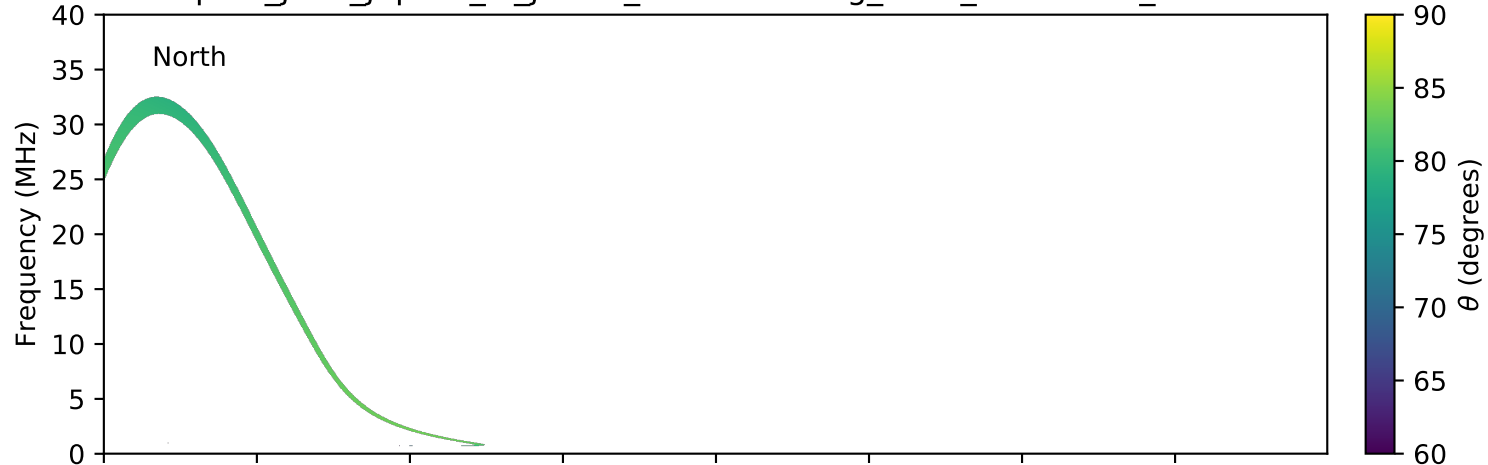
expres_juno_jupiter_io_jrm09_lossc-wid1deg_3kev_20211103_v11.cdf
