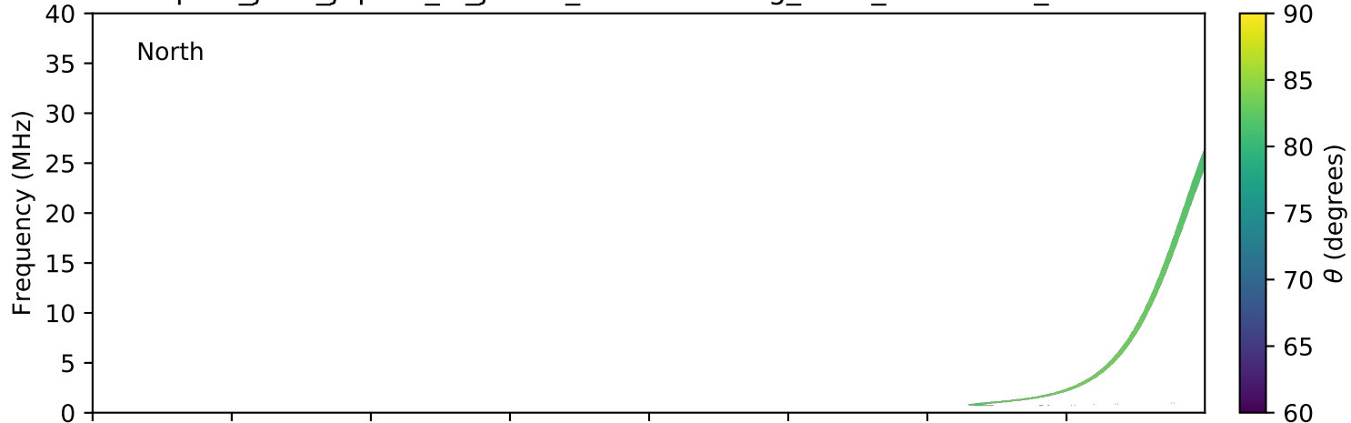
expres_juno_jupiter_io_jrm09_lossc-wid1deg_3kev_20211102_v11.cdf
