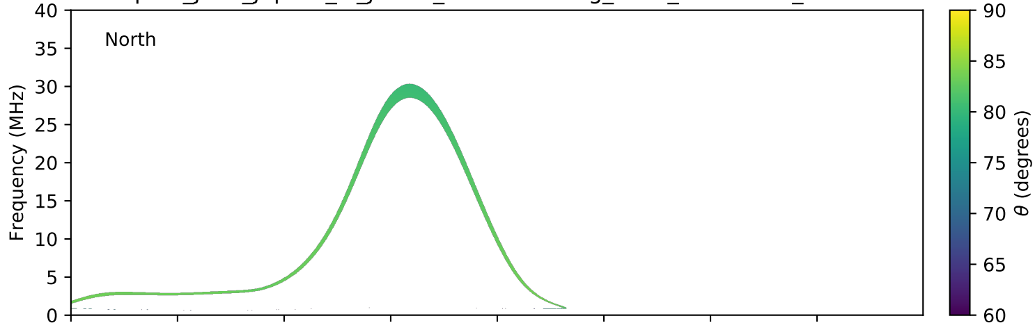
expres_juno_jupiter_io_jrm09_lossc-wid1deg_3kev_20211101_v11.cdf
