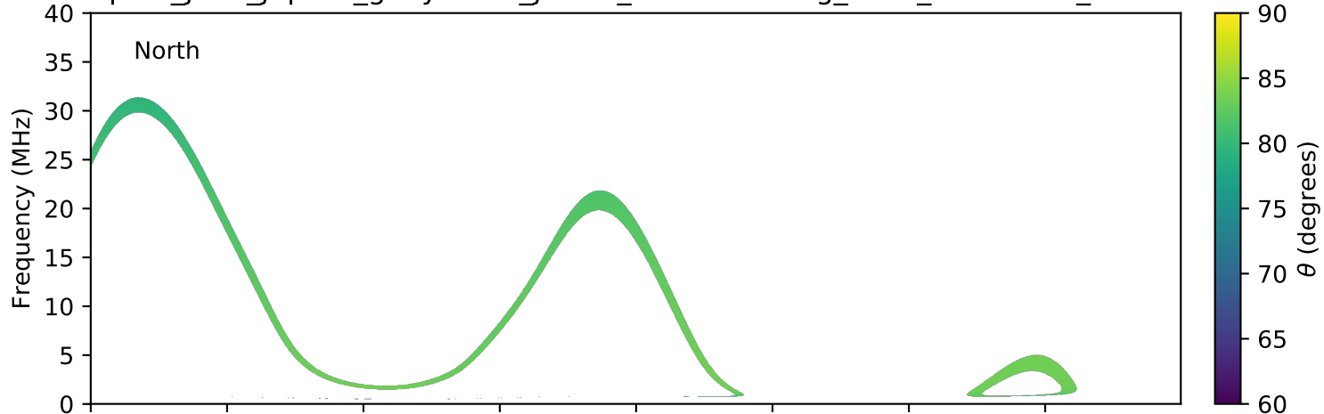
expres_juno_jupiter_ganymede_jrm09_lossc-wid1deg_3kev_20211127_v11.cdf
