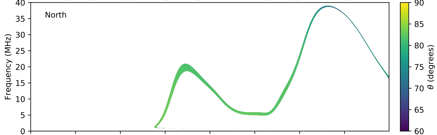
expres_juno_jupiter_europa_jrm09_lossc-wid1deg_3kev_20211127_v11.cdf
