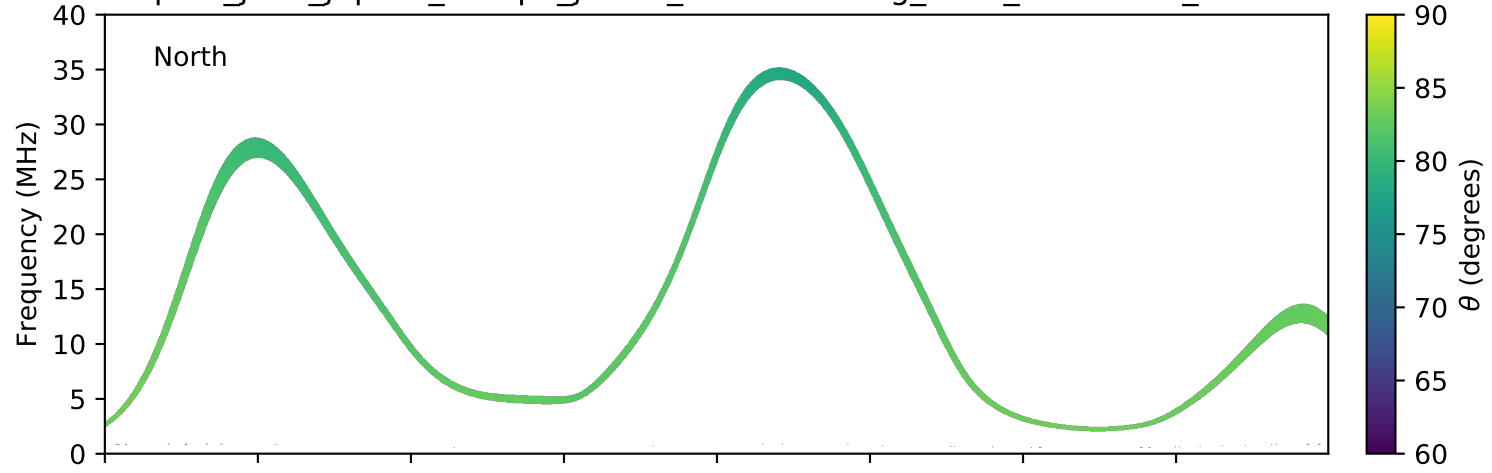
expres_juno_jupiter_europa_jrm09_lossc-wid1deg_3kev_20211124_v11.cdf
