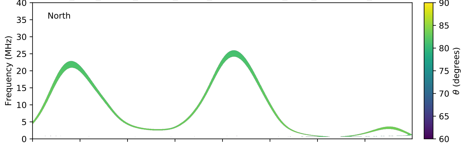
expres_juno_jupiter_europa_jrm09_lossc-wid1deg_3kev_20211117_v11.cdf
