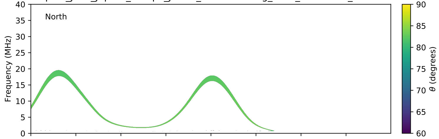
expres_juno_jupiter_europa_jrm09_lossc-wid1deg_3kev_20211110_v11.cdf
