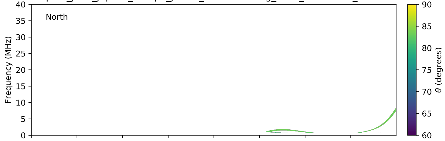
expres_juno_jupiter_europa_jrm09_lossc-wid1deg_3kev_20211109_v11.cdf
